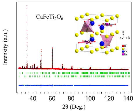
FIG. 1. (Color online) The powder XRD pattern of CFTO at room temperature and the results of Rietveld refinement with the space group P4_2/nmc (No. 137): a tiny amount impurity of \text{TiO}_2 ( \sim 2\% ) was observed; a peak in the range of 82^\circ to 83^\circ from the sample holder is excluded; the insert panel shows the crystal structure of CFTO.
