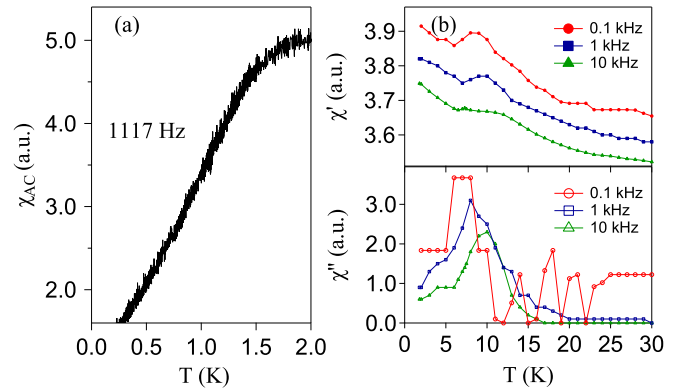
FIG. 5. (Color online) (a) Temperature dependence of ac susceptibility below 2 K measured in a ^3\text{He} refrigerator. (b) Temperature dependence of ac susceptibility (real part \chi' and imaginary part \chi'' ) at different frequencies from 1.8 K to 30 K of CFTO. \chi'' at 0.1 kHz is noisy because the signal is too low to be picked up by the lock-in amplifier at the highest gain.
