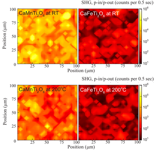
FIG. 2. (Color online) SHG micrographs on CFTO and CMTO: top panels were measured at room temperature, and the bottom panels at 200 °C. The average SHG of CFTO was very weak (around 170 counts at room temperature) and nearly temperature independent; whereas two orders of magnitude stronger SHG was observed in CMTO and the intensity was decreased by a factor of four with increasing temperature.
