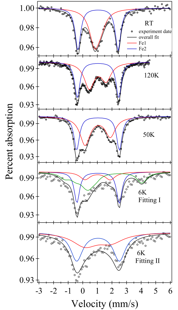
FIG. 7. (Color online) Mössbauer spectroscopy of CFTO at different temperatures. The open circles are experimental data and black solid lines are the overall fit to the data from the subcomponents shown; the red and blue solid lines are fittings for the hyperfine interactions at the tetrahedral Fe1 site and coplanar Fe2 site, respectively; the green solid line represents a residual component in addition to the contribution from QS at 6 K, see the text for detailed information about analyzing MS data.
