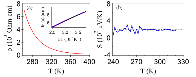
FIG. 9. (Color online) Temperature dependence of (a) resistivity \rho(T) and (b) thermoelectric power S(T) for CFTO.
