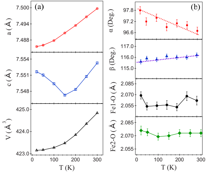
FIG. 3. (Color online) Temperature dependence of (a) lattice parameters and volume (most error bars are smaller than the symbols used in these plots). (b) Local interatomic distances and bond angles in CFTO.
