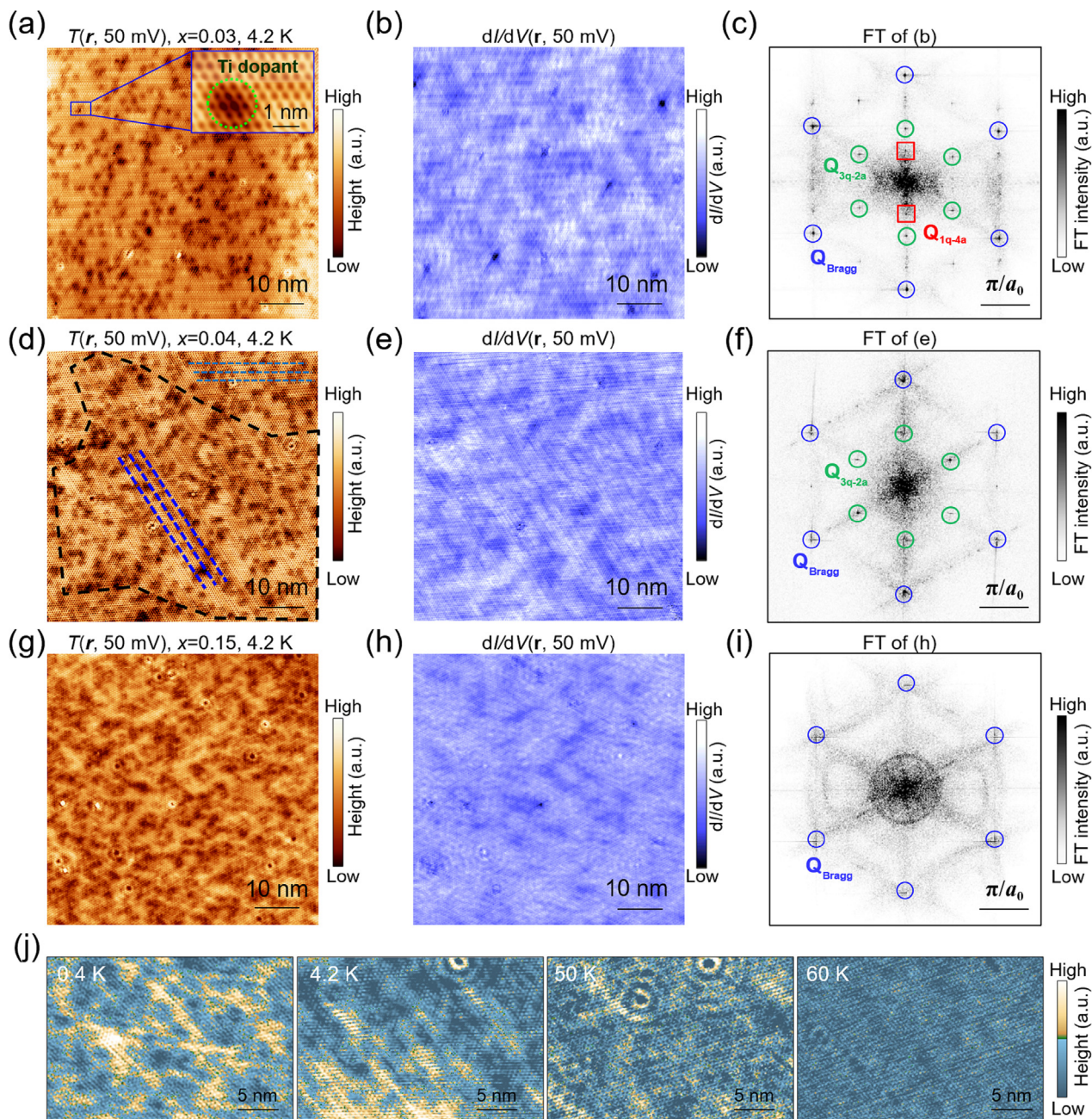
Fig. 3. Local electronic structures of CsV 3-x Ti x Sb 5 crystals. (a–c) STM topography (a), dI/dV(r, 50 \text{ mV}) (b) and the corresponding drift-corrected Fourier transform (FT) (c) at the large-scale Sb surface of CsV 3-x Ti x Sb 5 ( x = 0.03 ) obtained at 4.2 K, showing the 3Q-2a and 1Q-4a CDWs. Many dark spots, correlated to the Ti atoms, appear in the STM image of (a). The inset in (a): Zoom-in STM image showing the continuous lattice around the dark spots. (d–f) STM topography (d), dI/dV(r, -5 \text{ mV}) (e) and the corresponding drift-corrected FT (f) at the large-scale Sb surface of CsV 3-x Ti x Sb 5 ( x = 0.04 ), showing the presence of short-range 1Q-4a CDW multiple domains. Two 4a CDW domains can be clearly observed (highlighted by blue and light blue dotted lines). (g–i) STM topography (g), dI/dV(r, 50 \text{ mV}) (h) and the corresponding drift-corrected FT (i) at the large-sized Sb surface of CsV 3-x Ti x Sb 5 ( x = 0.15 ), showing the absence of 3Q-2a, and long-range 1Q-4a CDW states in the FT. The weak and elongated stripes around M points in (i) result from QPI pattern instead of long-range 3Q-2a CDWs. Setting parameter: tunneling current setpoint I_t = 1.0 \text{ nA} . (j) STM images of the Sb surface of CsV 3-x Ti x Sb 5 ( x = 0.15 ) at 0.4, 4.2, 50, and 60 K, respectively, showing that the short-range charge orders disappear at a critical temperature of \sim 60 \text{ K} . v_s = -50 \text{ mV} , I_t = 1.0 \text{ nA} .
