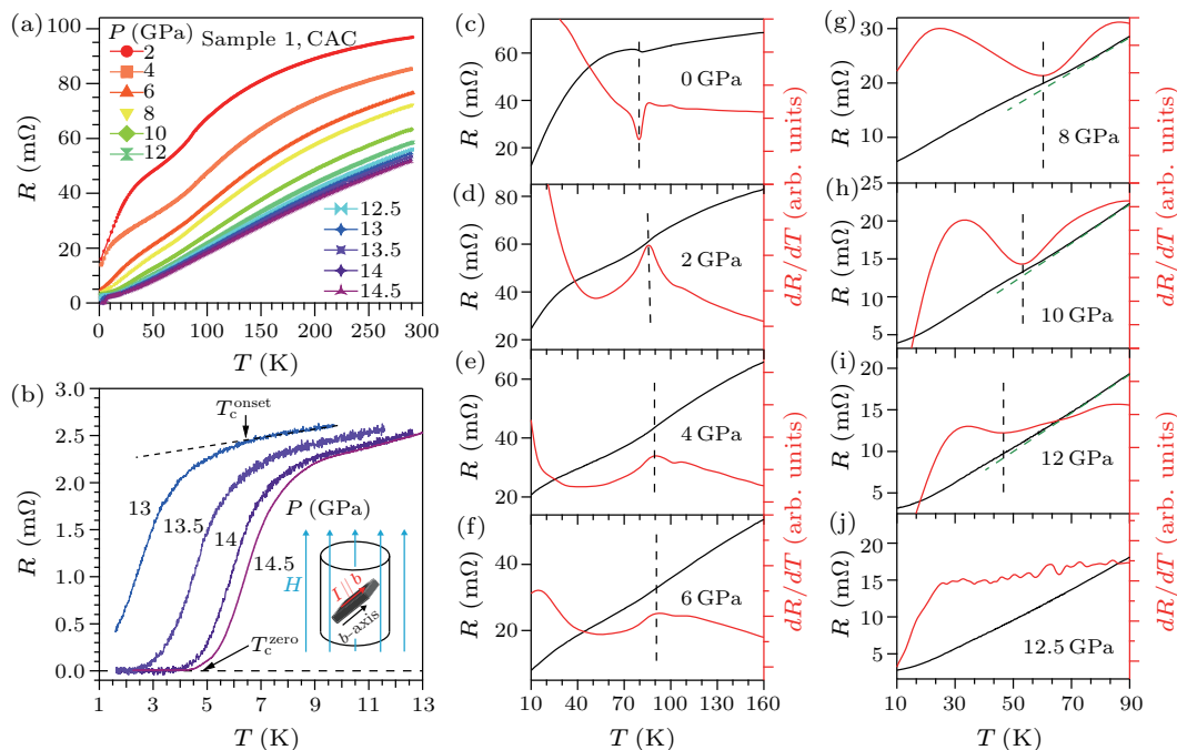
Fig. 2. (a) Electrical resistance of \text{RbMn}_6\text{Bi}_5 (sample 1) under various pressures measured in a CAC. (b) The low-temperature R(T) data highlighting the superconducting transition. (c)–(j) The R(T) and the corresponding dR/dT curve at each pressure showing the evolution of the antiferromagnetic transition.
