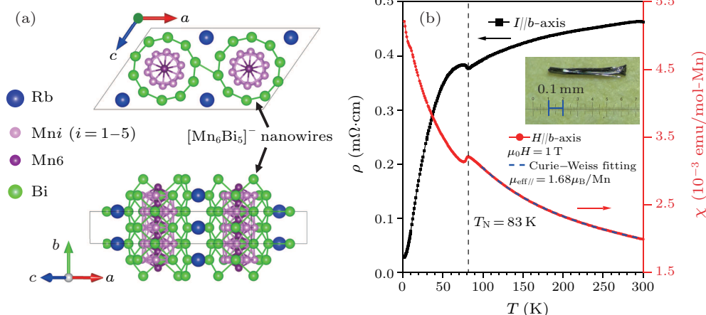
Fig. 1. (a) Crystal structure of \text{RbMn}_6\text{Bi}_5 . (b) Temperature dependence of the resistivity and magnetic susceptibility along the rod direction of \text{RbMn}_6\text{Bi}_5 crystal at AP. The T_N shows the antiferromagnetic transition temperature. The Curie-Weiss fitting is shown by the broken line. Inset of (b) shows a picture of the \text{RbMn}_6\text{Bi}_5 crystal.
