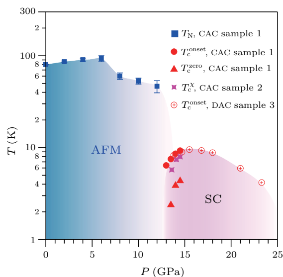
Fig. 4. T - P phase diagram of RbMn 6 Bi 5 . The AFM and SC refers to the antiferromagnetic and the superconducting phases, respectively.
