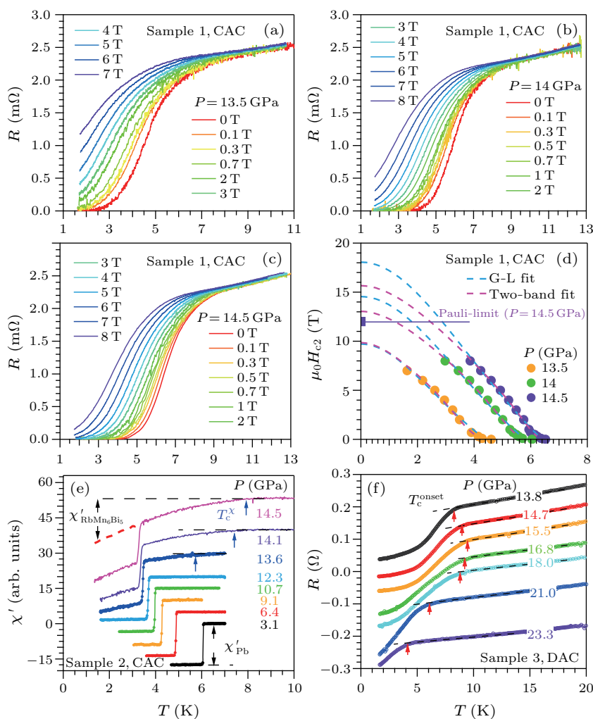
Fig. 3. (a)–(c) R(T) under different magnetic fields at 13.5, 14 and 14.5 GPa. (d) The temperature dependences of \mu_0 H_{c2}(T) fitted by the Ginzburg–Landau (G-L) equation, \mu_0 H_{c2}(T) = \mu_0 H_{c2}(0)[1 - (T/T_c)^2]/[1 + (T/T_c)^2] and the two-band model. (e) The ac magnetic susceptibility \chi'(T) of RbMn 6 Bi 5 crystal (sample 2) and a piece of Pb with similar volume. (f) The low-temperature R(T) data of RbMn 6 Bi 5 crystal (sample 3) measured with a DAC. The curves in (e) and (f) have been shifted vertically for clarity.
